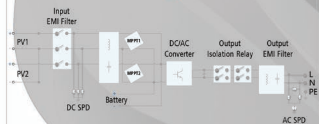
Circuit Diagram
